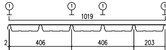
Klip-Lok 406 SMD360M-6X12UW
